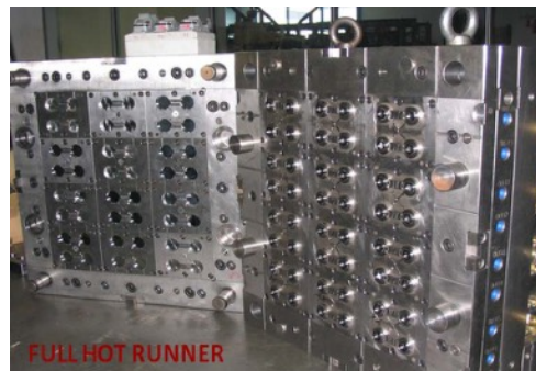
Plastic Molding
