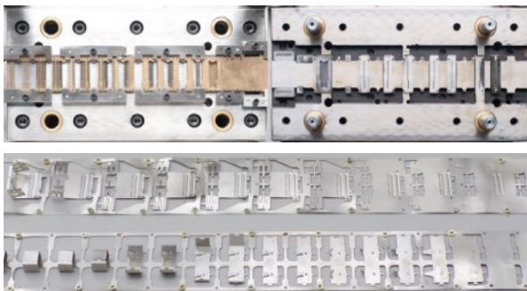
Contacts & Shield Stamping
